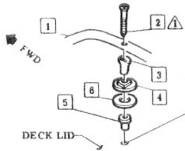
VIEW A TYPICAL (8 PLACES)
